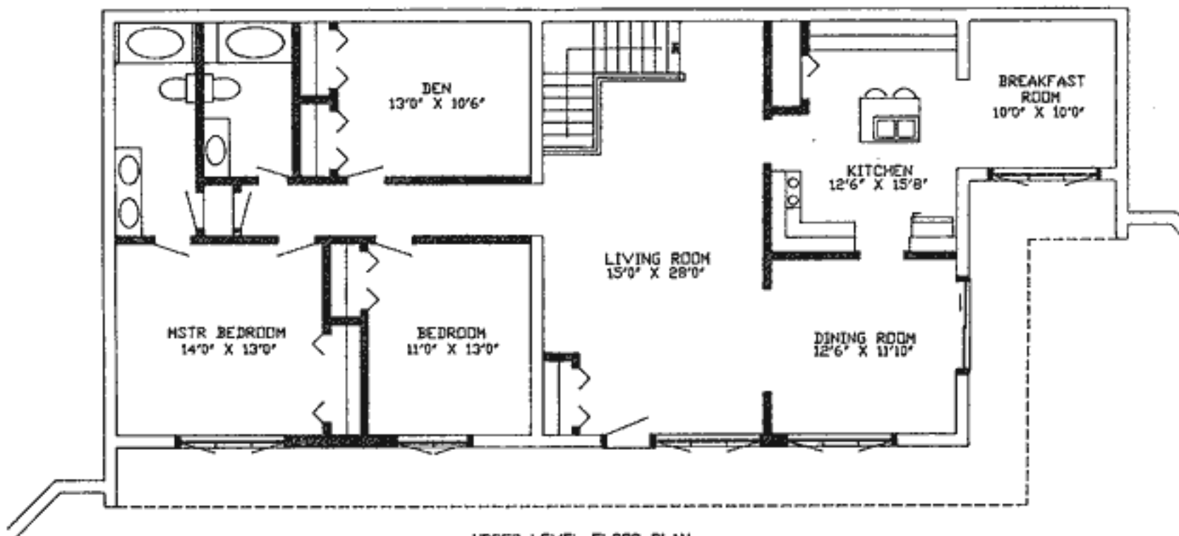
UPPER LEVEL FLOOR PLAN
